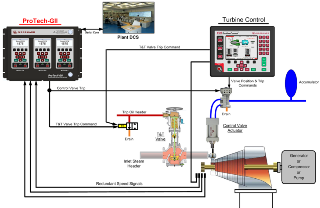
2-out-of-3 Voted Application Diagram
